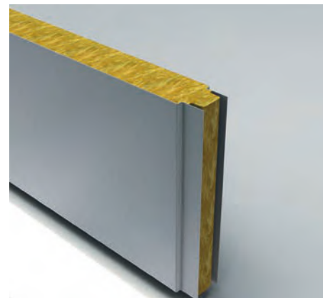
Mineral Wool
