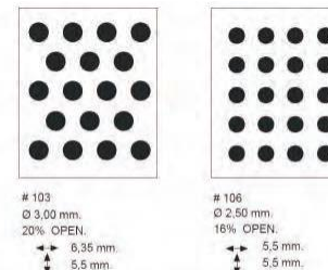
PERFORATION DETAILS :
