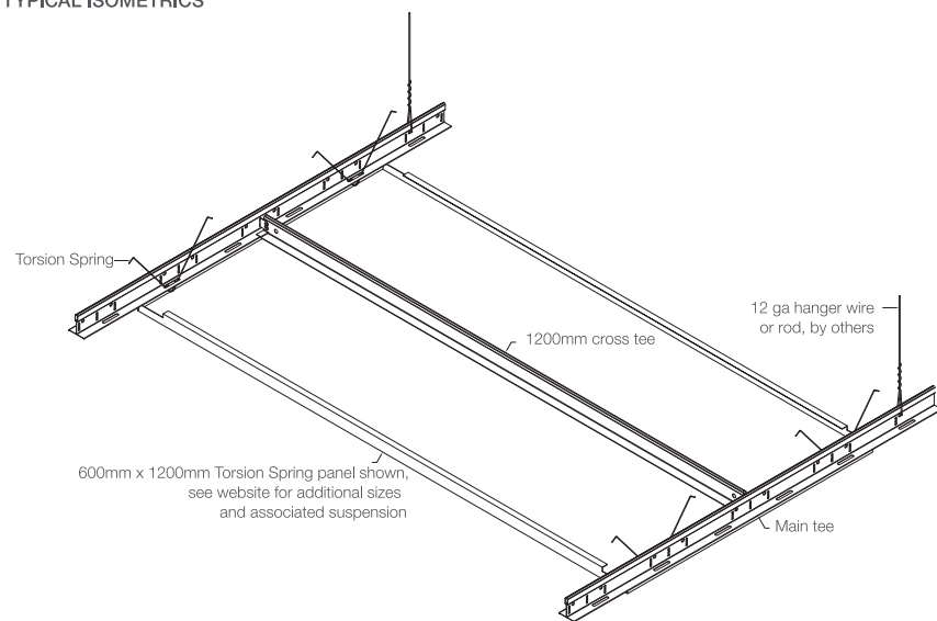
TYPICAL ISOMETRICS
